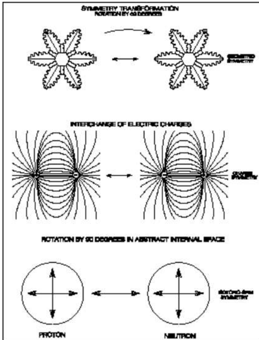
Figure 6. Symmetries of nature determine the properties of forces in Gauge theories. The symmetry of a snowflake can be characterized by noting that the pattern is unchanged when it is rotated 60 degrees; the snowflake is said to be invariant with respect to such rotations. In physics, non-geometric symmetries are introduced. Charge symmetry, for example, is the invariance of the forces acting among a set of charged particles when the polarities of all the charges are reversed. Isotopic-spin symmetry is based on the observation that little would be changed in the strong interactions of matter if the identities of all protons and neutrons were interchanged. Hence proton and neutron become merely the alternative states of a single particle, the nucleon, and transitions between the states can be made (or imagined) by adjusting the orientation of an indicator in an internal space. It is symmetries of this kind, where the transformation is an internal rotation or a phase shift, which are referred to as Gauge symmetries.
