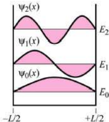
Figure 3a. The three lowest wave functions, \psi(x) , \psi_1(x) , \psi_2(x) , of an infinite quantum well.
