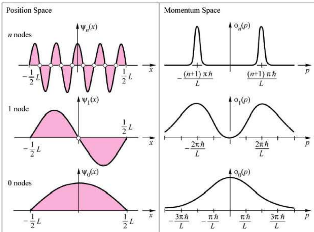
Figure 3b. Position space representation and momentum space representation of three wave functions \psi(x) , \psi_1(x) , \psi_n(x) . The subscript n refers to the number of nodes (nodes at x = \pm 1/2L are not counted).
